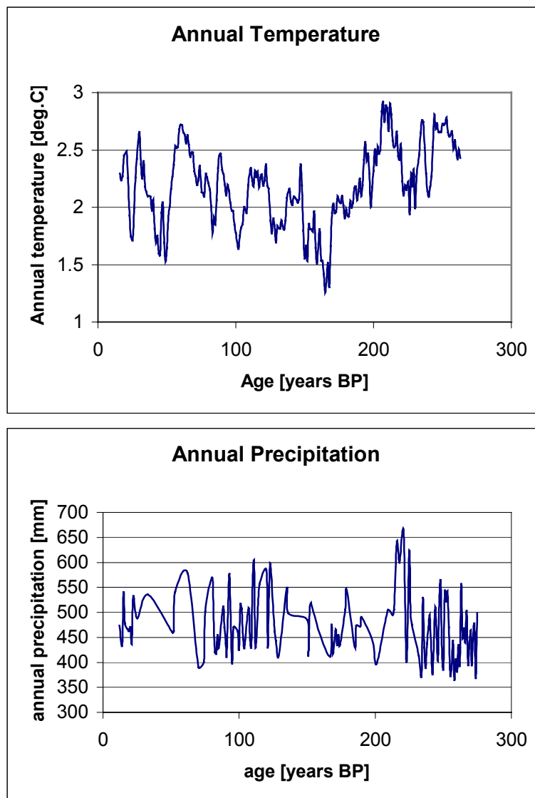
Fig.3 (Up) Annual temperature in the last 280 years for Kananaskis country, Alberta, Canada derived from annual intensity of luminescence of a stalagmite from Rats Nest cave, Alberta, Canada
